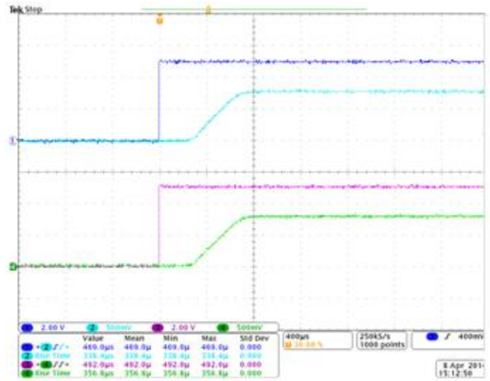
Turn ON Response Time V_{\text{IN}}=0.8\text{V} , V_{\text{BIAS}}=5\text{V} , C_{\text{IN}}=1\mu\text{F} , C_{\text{L}}=0.1\mu\text{F} , C_{\text{SS}}=1\text{nF} , R_{\text{L}}=10\Omega
